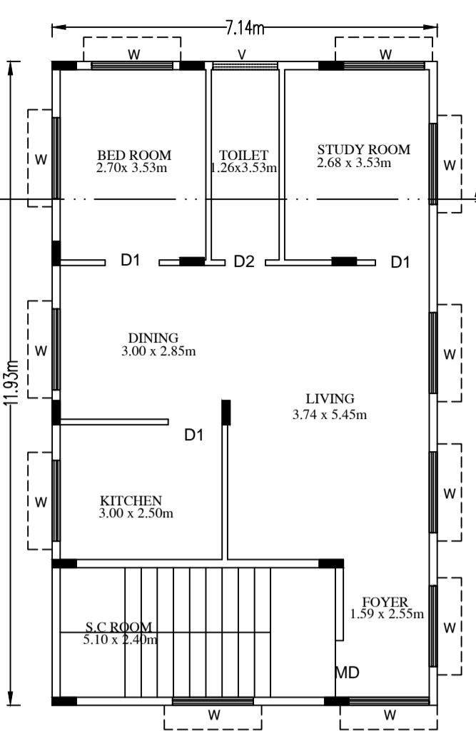
PROPOSED TYPICAL FIRST & SECOND FLOOR PLAN
